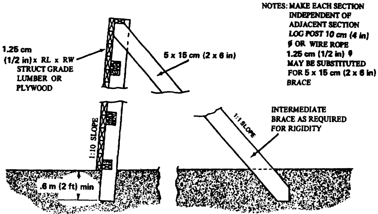
Figure 1-41. Wooden standoff.
